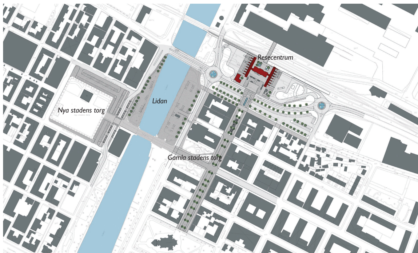
Situationsplan
